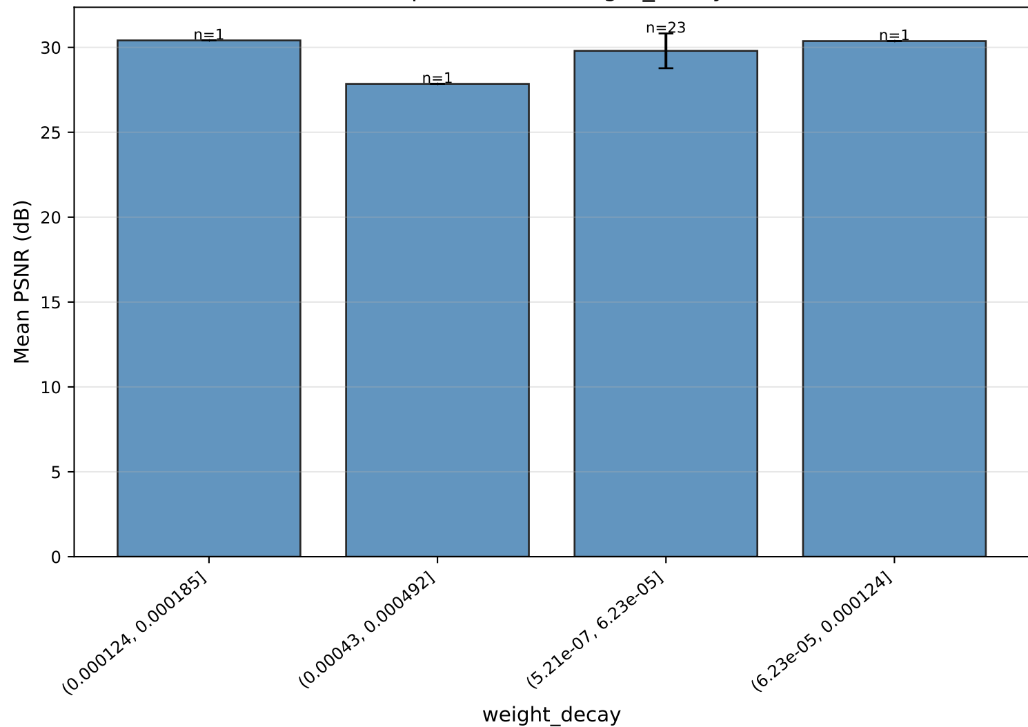
Mean PSNR per value of weight_decay — SwinT
